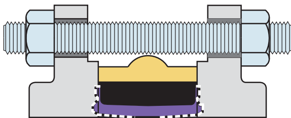
Wafer valve connection.
