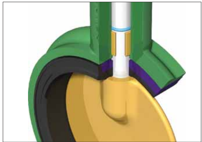
Hard-backed cartridge seat.
