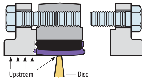
Lug valve connection with downstream flange removed.
